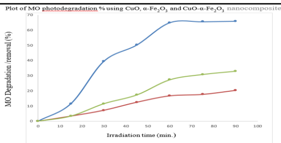
Figure 7. Plot of comparative study of CuO , \alpha - Fe_2O_3 and CuO - \alpha - Fe_2O_3 Photocatalysis
