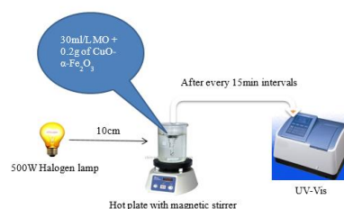
Figure 3: experimental set up for the Photocatalytic degradation of MO dye.
