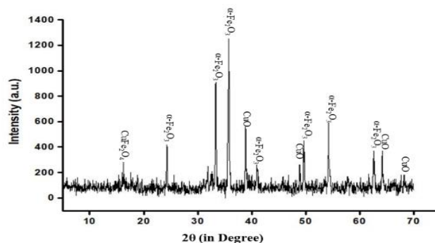
Figure 4. X-ray diffraction spectrum (XRD) of the \text{Cu}-\alpha\text{-Fe}_2\text{O}_3 nanocomposite
