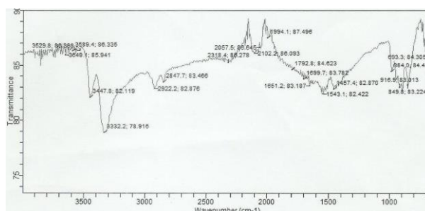
Figure 6: FTIR spectrum of the \text{CuO}-\alpha\text{-Fe}_2\text{O}_3 showing the absorption peaks
